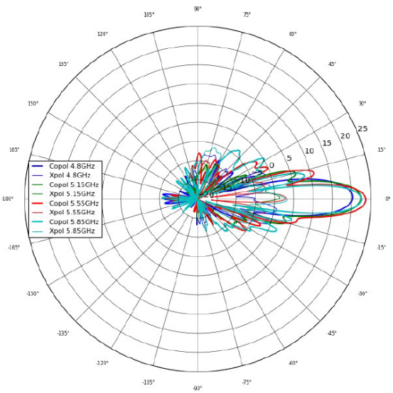
Elevation Vertical
